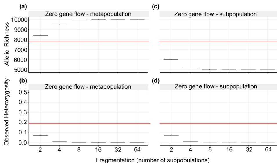
FIGURE 2 Allelic richness (number of alleles retained from original 10,000) and observed heterozygosity from 50 replicate simulations of unlinked neutral loci in a "meta"population (a and b) and in a single subpopulation (c and d) under various levels of fragmentation and zero gene flow (Scenario 2). Red horizontal line represents the values obtained in Scenario 1.
