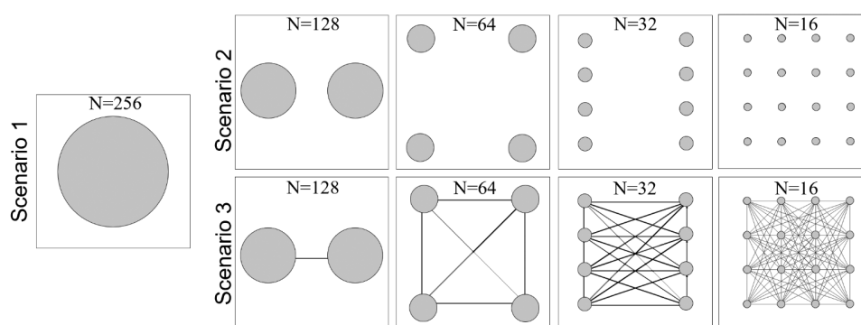
FIGURE 1 Representation of Scenarios 1–3. Scenario 1 is a single panmictic population. In Scenarios 2 and 3, fragmentation increases from left to right. Scenario 2 has zero gene flow between subpopulations (Table 1). Rates and frequency of gene flow in Scenario 3 (grey lines) vary as per Table 1. The total number of individuals in all simulated scenarios is 256 and the number of individuals per subpopulation is shown. For brevity, fragmentation above 16 subpopulations is not shown.
