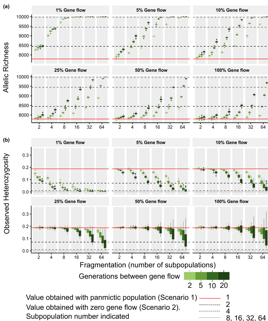
FIGURE 3 Allelic richness (number of alleles retained from original 10,000; a) and observed heterozygosity (b) from simulations of unlinked neutral SNP loci in a metapopulation undergoing episodic fragmentation and mixing (Scenario 3). Results are drawn from 50 replicate simulations using output from every generation between the last generation in which gene flow occurred to generation 500. Horizontal lines represent values obtained in Scenario 1 (red) and Scenario 2 with no gene flow (black dashed, two subpopulations; dark grey dashed, four subpopulations; mid-grey dashed, eight, 16, 32 and 64 subpopulations).
