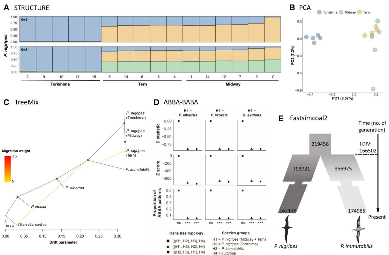
FIG. 3. Population structure and gene flow in tropical albatrosses. (A) Population structure of P. nigripes inferred by STRUCTURE ( K = 2 and 3 ). Assignment probabilities of individuals to one or other cluster(s) are indicated on the y-axis. Individual IDs are indicated on the x-axis along with their population of origin. (B) PCA for P. nigripes individuals. (C) Gene flow among albatross species detected by TreeMix. The migration weight represents the fraction of ancestry derived from the migration edge. Green circle on node indicates bootstrap support >90\% . (D) Introgression inferred by ABBA-BABA tests between P. nigripes populations and P. immutabilis using three different outgroup species. The test significance is indicated on the x-axis following P -values as follows: ***P < 0.001 , **P < 0.01 , *P < 0.05 , and (ns) nonsignificant. Detailed results are given in the supplementary table S1, Supplementary Material online . (E) Divergence of P. nigripes and P. immutabilis reconstructed by Fastsimcoal2. Numbers represent effective population size or generation number (not to scale). Detailed results are given in the supplementary figure S7, Supplementary Material online . Illustrations reproduced with permission of Lynx Edicions. s.e., standard error.
