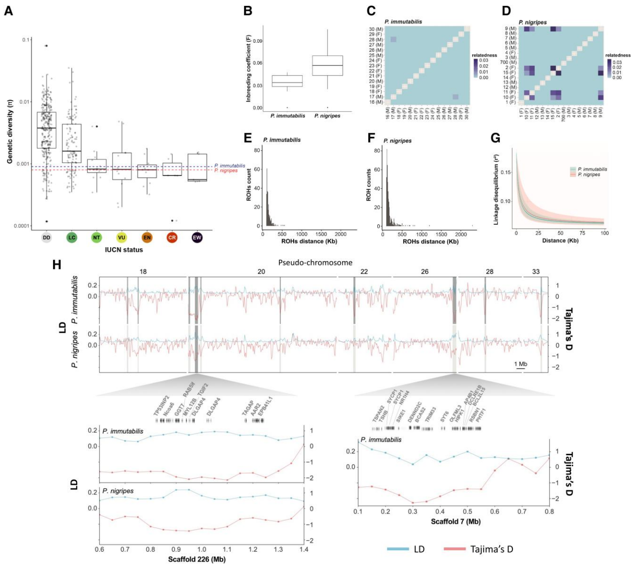
FIG. 6. Genetic diversity ( \pi ), inbreeding coefficients, genetic relatedness, ROHs distribution, LD, and selective sweeps of Phoebebastris immutabilis and P. nigripes . (A) Genetic diversity ( \pi ) assessed across species of different IUCN categories. Genetic diversity data are adopted from Robinson et al. (2016). The genetic diversities estimated for P. immutabilis and P. nigripes are highlighted by horizontal dotted lines. Both albatross species are currently classified as near threatened. (B) Inbreeding coefficient of P. immutabilis and P. nigripes . Genetic relatedness among pairwise individuals of (C) P. immutabilis and (D) P. nigripes . Distribution of ROHs for (E) P. immutabilis and (F) P. nigripes based on unlinked SNPs, with minimum windows sizes of 50 SNPs and 1 kb, allowing for five missing sites and five heterozygous sites. (G) LD decay based on the r^2 index. (H) Signal of selective sweep in P. immutabilis and P. nigripes . Each genome was scanned for regions with outliers of high LD and low Tajima's D, along sliding-windows of 100 kb size and 50 kb step. The LD (upper blue lines) and Tajima's D (lower red lines) values are shown on the left and right y-axes, respectively. Pseudochromosomes (top panel) and scaffolds (bottom panel) are shown on the x-axis. Only pseudochromosomes 18, 20, 22, 26, 28, and 33 are shown here. Candidate genomic windows with signature of selective sweeps are highlighted in dark gray. The largest candidate windows (300–450 kb), located on scaffolds 7 and 226, are shown in detail with their gene content. Positions on the scaffold are shown on the y-axis. DD, data deficient; LC, least concern; NT, near threatened; VU, vulnerable; EN, endangered; CR, critically endangered; EW, extinct in the wild.
