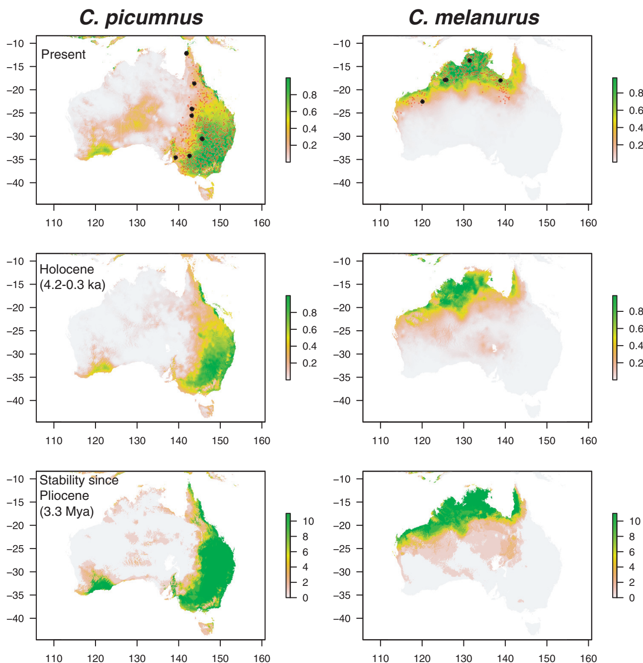
Figure 7. Environmental niche models of C. picumnus (left) and C. melanurus (right) for the present (top) and Holocene (middle) time periods. The niche stability since the Pliocene is depicted on the bottom row. In all panels, green indicates highest probability whereas brown and grey indicates lowest probability. x - and y -axes are longitude and latitude, respectively. Mya, millions of years ago; ka, thousands of years ago.
